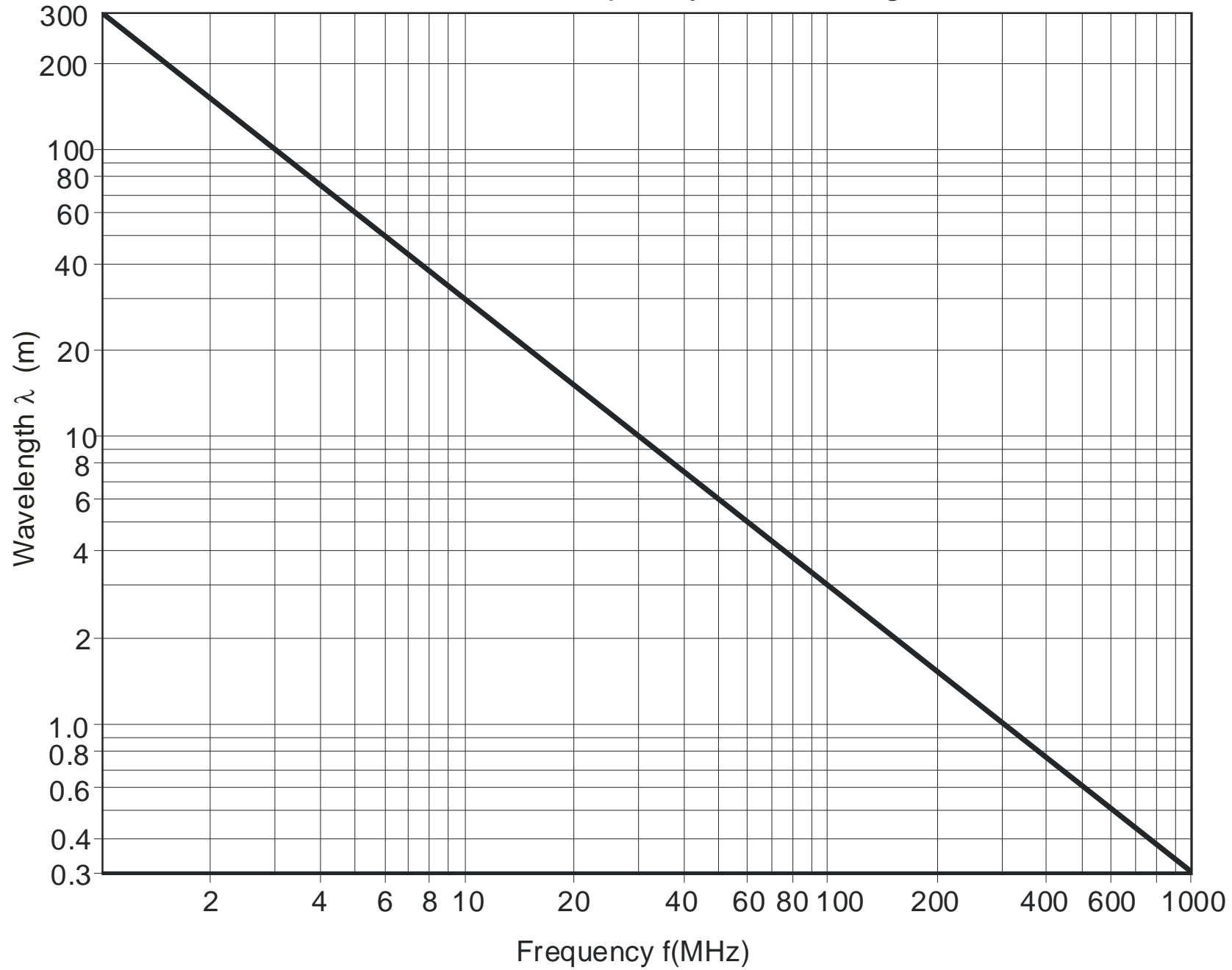
Conversion chart Frequency to Wavelength
